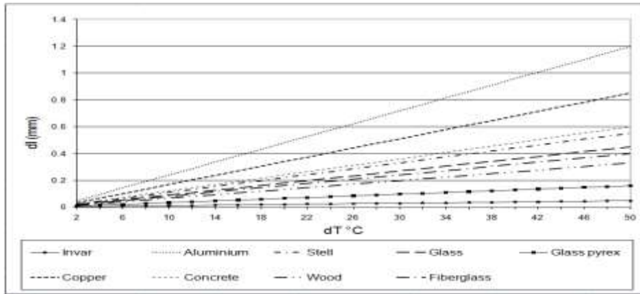
Fig 3. The change of l_m of several materials length in relation to the temperature change
