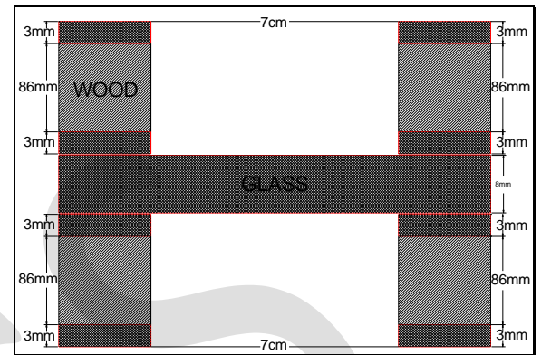
Fig 2. Enlargement of one comparator's step
