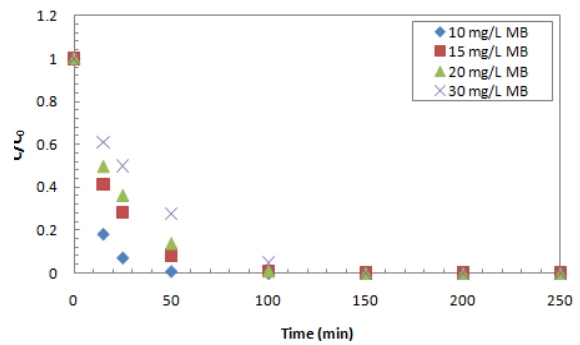
Fig. 8. The effect of 10, 15, 20 and 30 mg/L concentrations of methylene blue in the presence of 0.66 g ZnO/SnO 2 nanocomposite.
