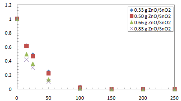
Fig. 12. The effect of 0.33, 0.50, 0.66 and 0.83 g amounts of ZnO/SnO 2 nanocomposite in the presence of 20 mg/L methylene blue.
