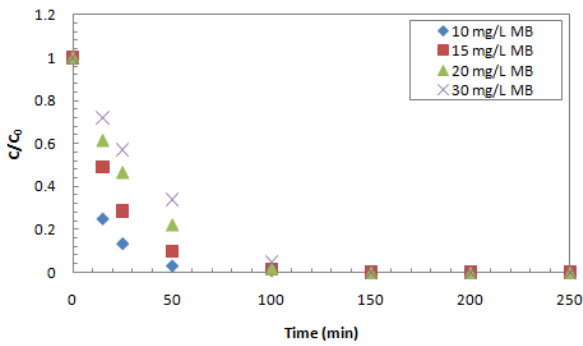
Fig. 7. The effect of 10, 15, 20 and 30 mg/L concentrations of methylene blue in the presence of 0.50 g ZnO/SnO 2 nanocomposite.
