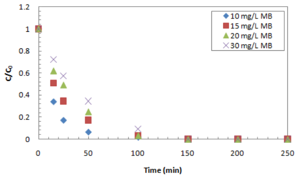
Fig. 6. The effect of 10, 15, 20 and 30 mg/L concentrations of methylene blue in the presence of 0.33 g ZnO/SnO 2 nanocomposite.
