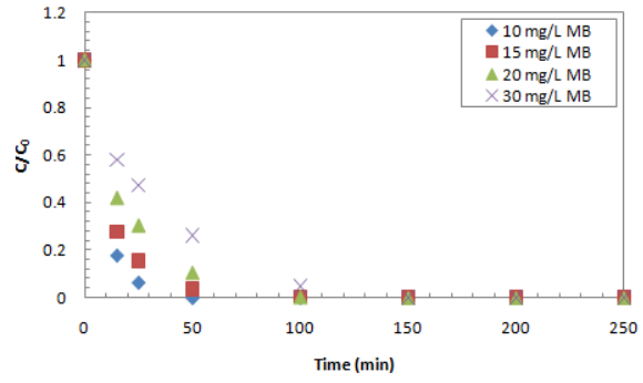
Fig. 9. The effect of 10, 15, 20 and 30 mg/L concentrations of methylene blue in the presence of 0.83 g ZnO/SnO 2 nanocomposite.
