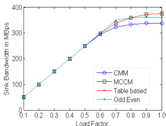
Figure 4. Sink Bandwidth at various Load factors
