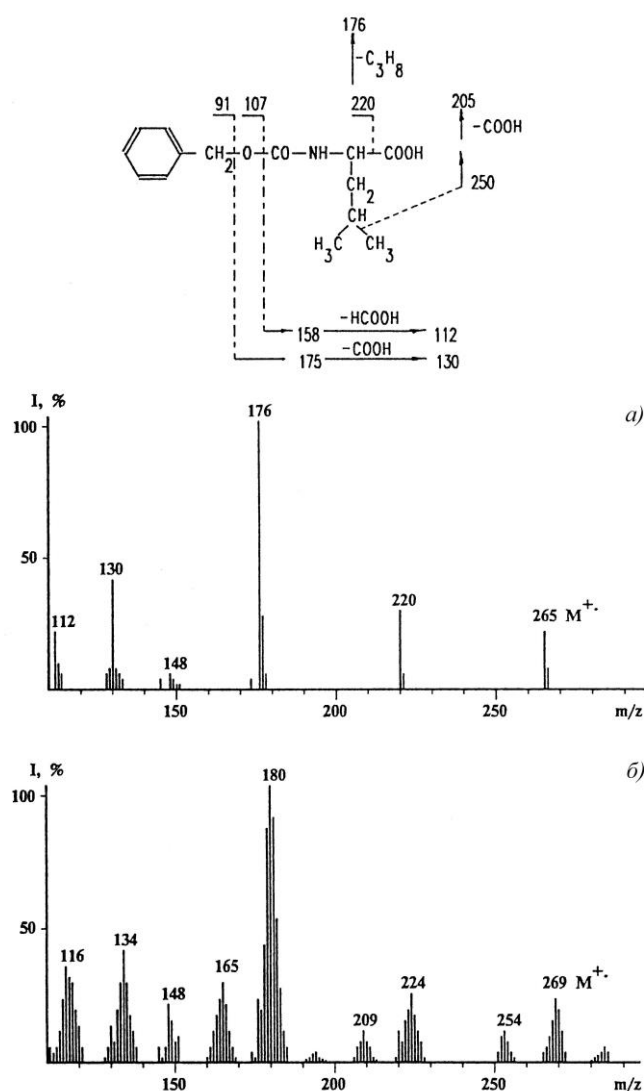
Fig. 3. EI mass spectra of N-Cbz- ^{13}\text{C} -Leu, isolated from liquid culture of M. flagellatum after the treatment by benzyloxycarbonyl: a – 1 % methanol and \text{H}_2\text{O} (the control); b – 1 % ^{13}\text{C} methanol and \text{H}_2\text{O} .
