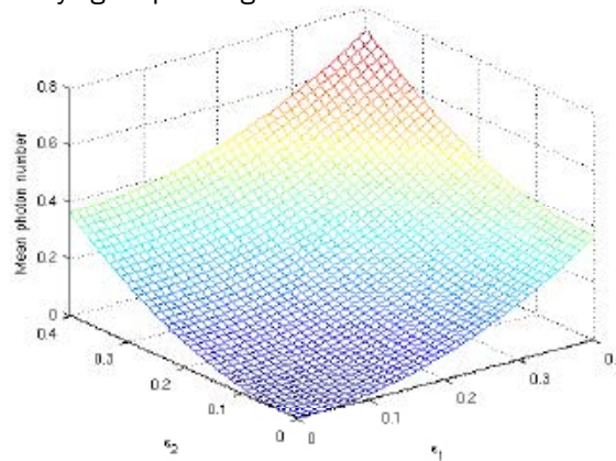
Figure 1: A plot of \bar{n} [Eq. 27] versus \varepsilon_1 and \varepsilon_2 for \kappa = 0.8 .
