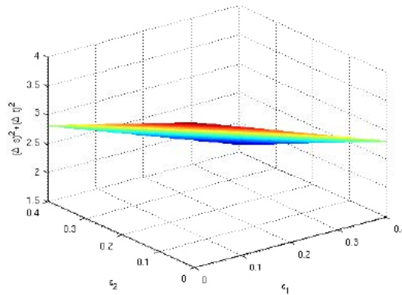
Figure 3: A plot of (\Delta s)^2 + (\Delta t)^2 [Eq. 63] versus \epsilon_1 and \epsilon_2 for \kappa = 0.8 .
