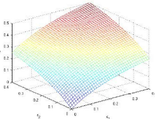
Figure 2: A plot of S_{+} [Eq. 49] versus \varepsilon_1 and \varepsilon_2 for \kappa = 0.8 .
