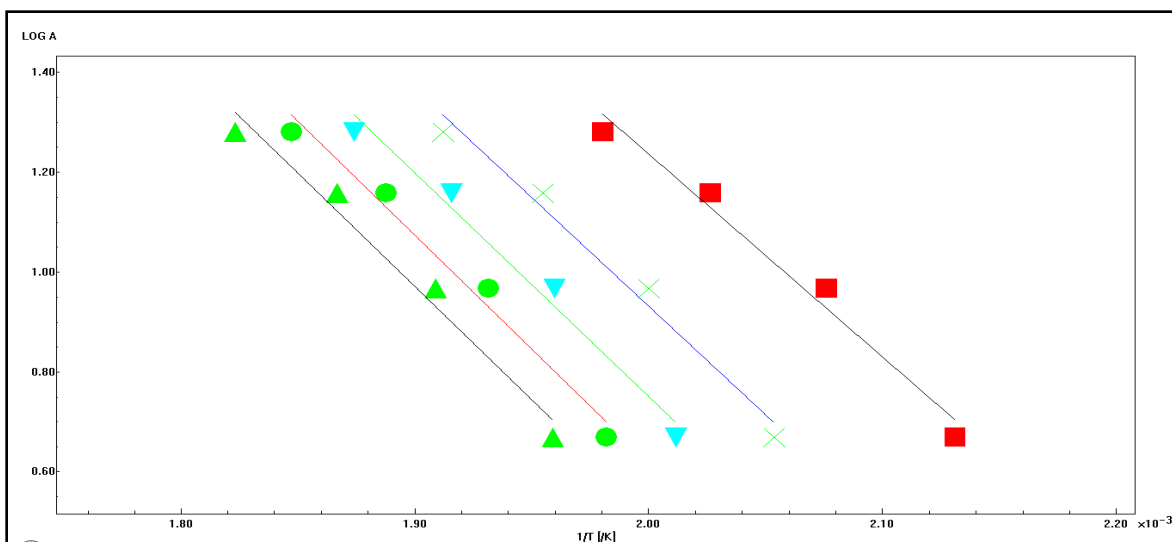
Fig.7: Ozawa curves of Cilostazol plot of log \beta again 1/T
