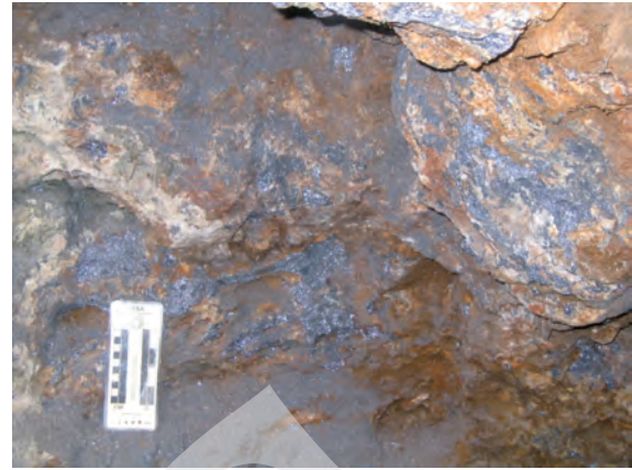
Figure 11. Photograph of brecciated limestone replaced by galena ore (grey in colour). Location Latong River.
