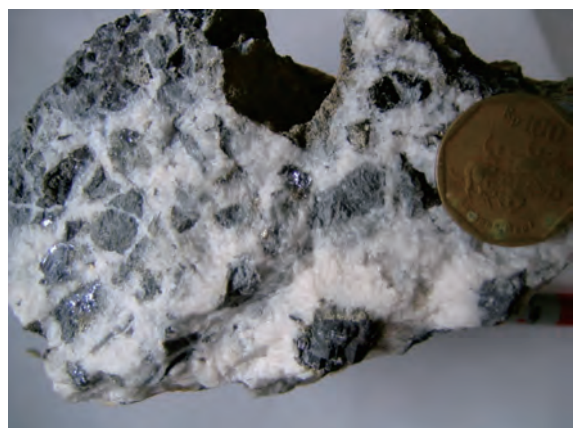
Figure 13. Photograph of marcasite and galena within the altered sericite-quartz veins.
