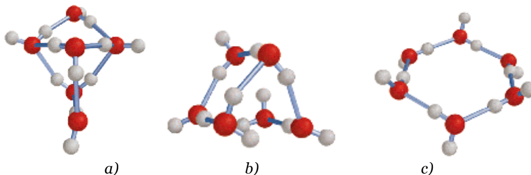
Figure 10. Calculation of small water cluster structures (a–c) with general formula (H 2 O) n , where n = 6 [29] (Tsai & Jordan, 1993).
