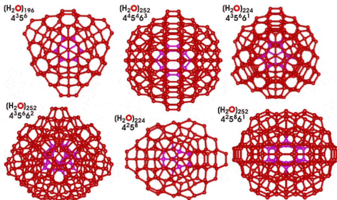
Figure 13. Tetrahedron water clusters (\text{H}_2\text{O})_n with different symmetry ( n = 196, 224, 252 ) [32].
