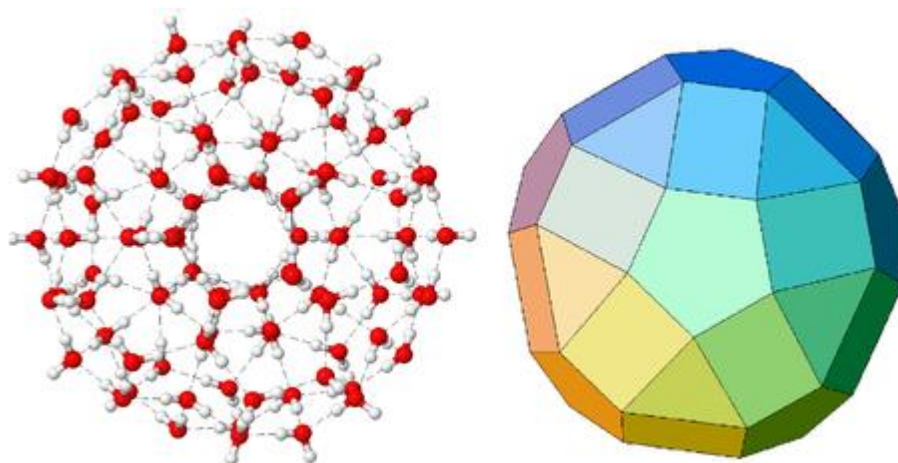
Figure 15. Icosahedron cluster based on 100 \text{H}_2\text{O} molecules and the underlying structure according to M. Chaplin.
