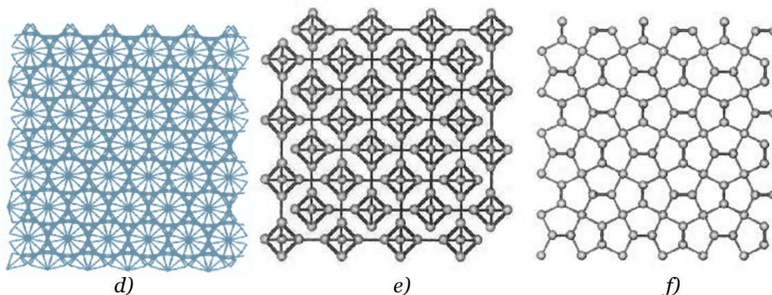
Figure 2. Ice crystalline modifications: a ) - natural hexagonal ice I_h ; b ) – ice of II configuration; c ) – ice of III configuration; d ) – ice of IV configuration; e ) – ice of VI configuration; f ) – ice of XII configuration.
