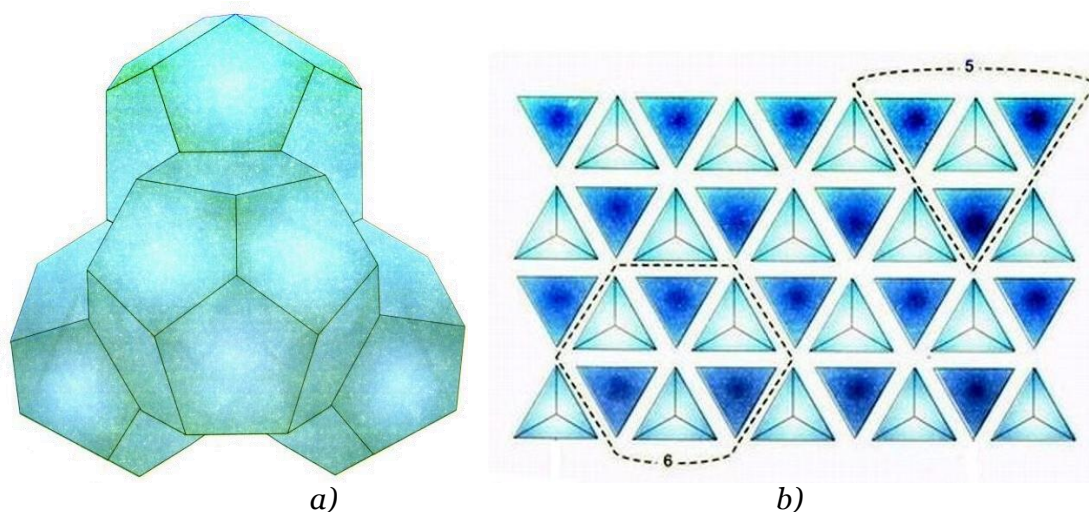
Figure 14. Model of water associates according to S.V. Zenin: a ) – associate of 57 H 2 O molecules, tetrahedron of four dodecahedron ("quantum"); b ) – bulk packaging of "quanta" (Zenin, 1999).
