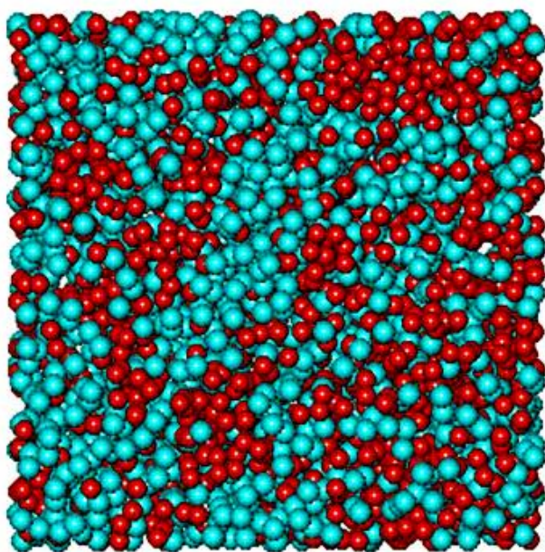
Figure 5. The model composing of 3456 water molecules at a temperature of 297 K. Red balls – H 2 O molecules with the low values of the Voronoi polyhedra volume (less than 26.33 Å), i.e. molecules in areas with a higher local density. Blue - molecules with the large volumes of values (more than 34.1 Å). It was selected by 25% of the molecules of each kind. It is evident that the molecules of each kind have a tendency to associate with each other, showing the scale of existing structural inhomogeneities in the water.
