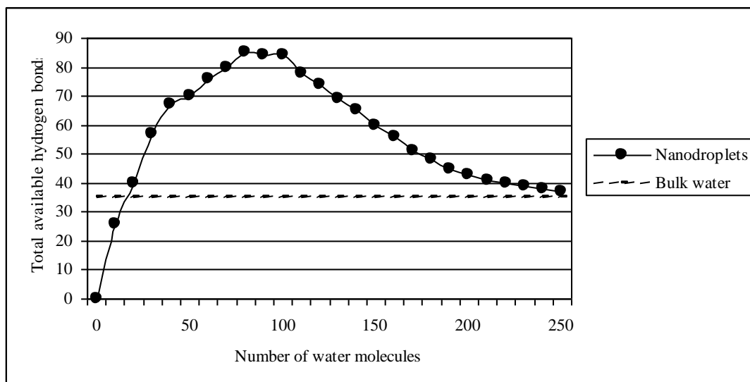
Figure 8. The total number of hydrogen bonds depending on the number of water molecules in clusters.
