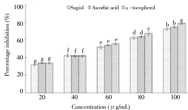
Figure 2. Nitric oxide radical scavenging activity of a diterpenoid sugiol from M. glyptostrobooides and standard antioxidants, ascorbic acid and \alpha -tocopherol.
