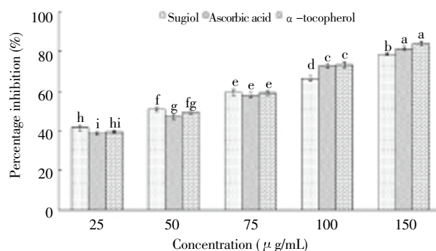
Figure 1. DPPH radical scavenging activity of a diterpenoid sugiol from M. glyptostrobooides and standard antioxidants, ascorbic acid and \alpha -tocopherol.
