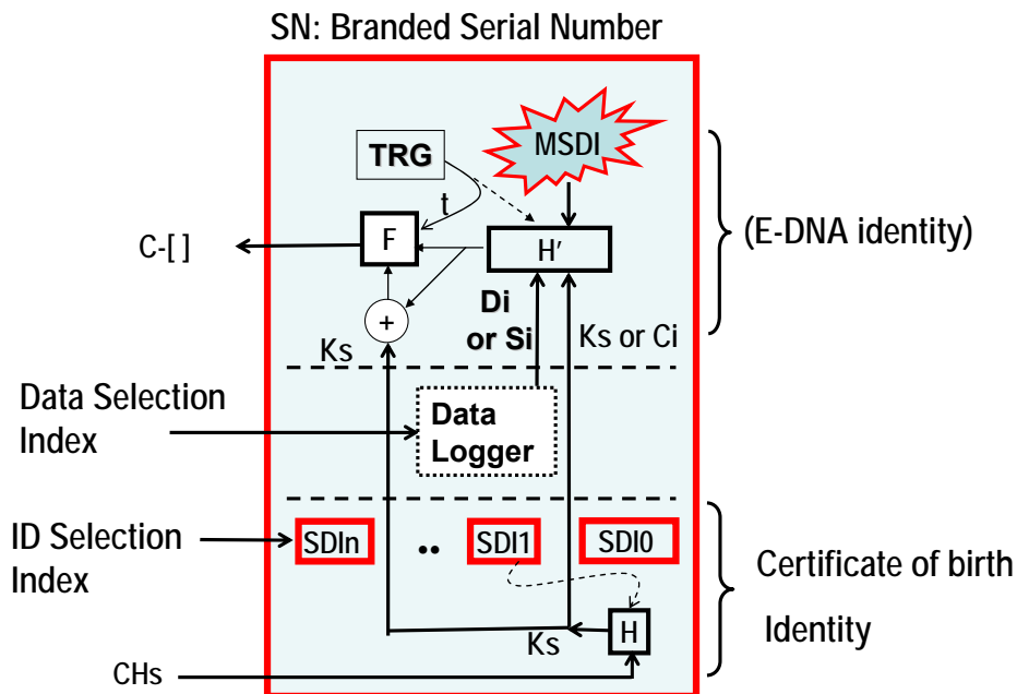
Figure 4. Hardware Core for a Living Identification Mechanism
