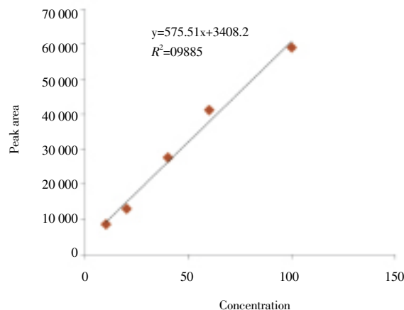
Figure 4. Standard calibration curve of quercetin.
