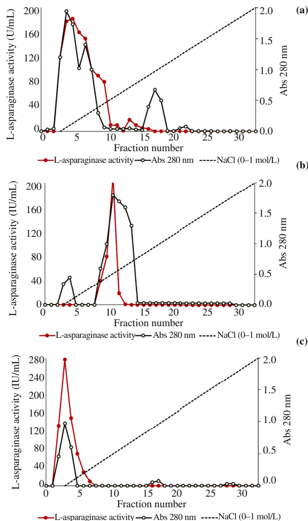
Figure 1. Chromatographic separation of L-asparaginase produced by A. oryzae CCT 3940.
