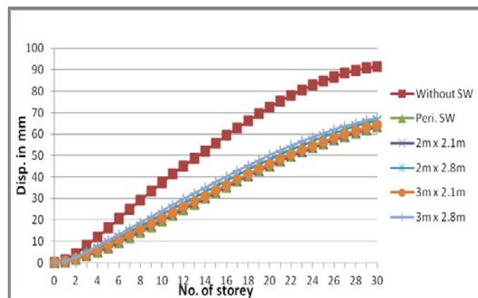
Figure 8: Displacement Comparison between different sizes of openings.
