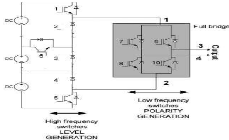
Fig. 2. Proposed circuit using RV topology
