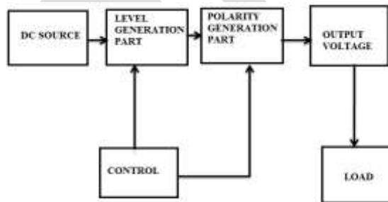
Fig.4.3: General Block Diagram of Seven Level proposed Topology
