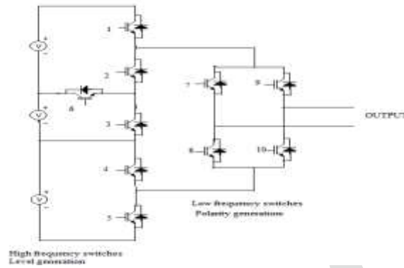
Fig. 1. General single phase multilevel inverter (using reverse voltage topology) circuit
