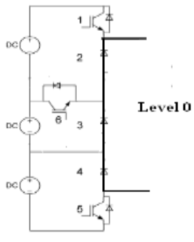
Fig. 3. Level 0 = 0 V dc
