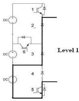
Fig. 4. Level 1 = V dc
