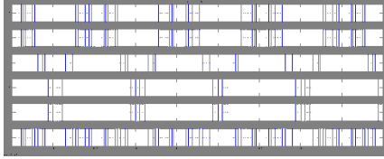
Fig. 10. Complete gate signals for seven-level generation
