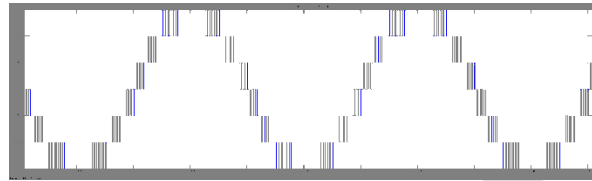
Fig. 12. Output voltage of polarity generation part
