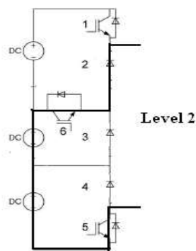
Fig. 5. Level 2 = 2V dc
