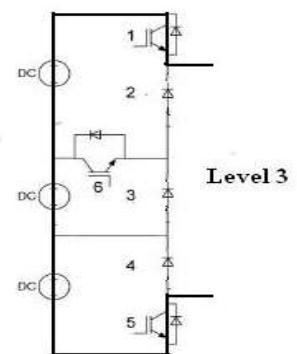
Fig. 6. Level 3 = 3 V dc
