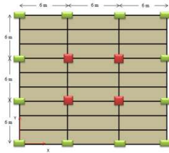
Figure 3.1: Plan of Building
