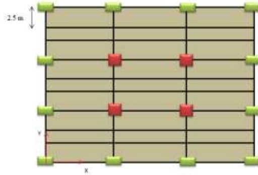
Figure 6.1: Models I - Slab with Main and Secondary Beam at Spacing 2.5 m
