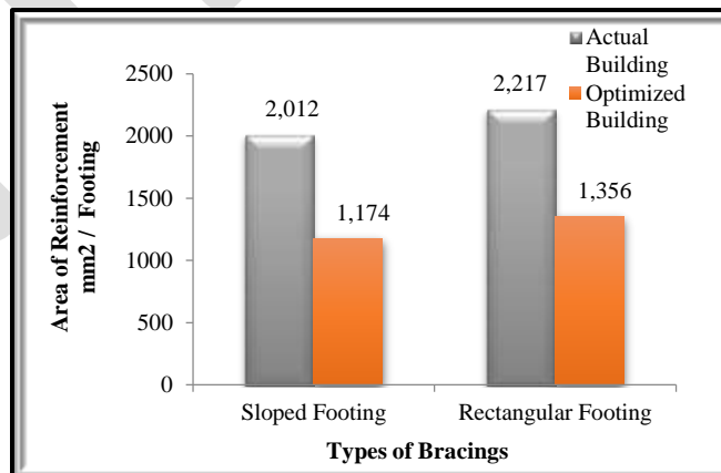
Graph 6.12: Total Area of Reinforcement for Types of Bracings
