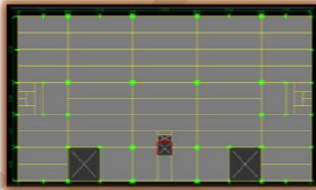
Figure 7.1: Plan of College Main Building
