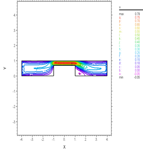
Fig.10: Velocity in x – direction at h = 0.7
