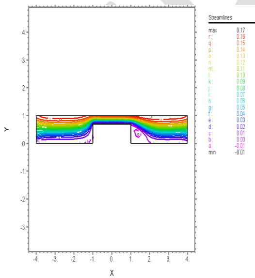
Fig.9: Streamlines at h = 0.7
