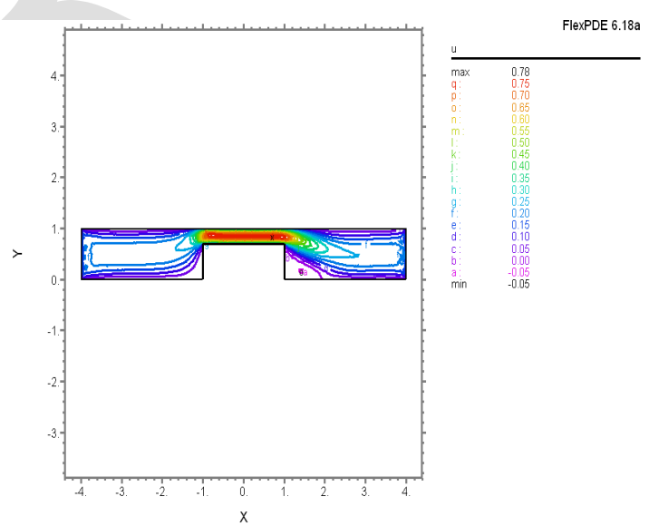
Fig.14:Velocity in x – direction at h = 0.9
