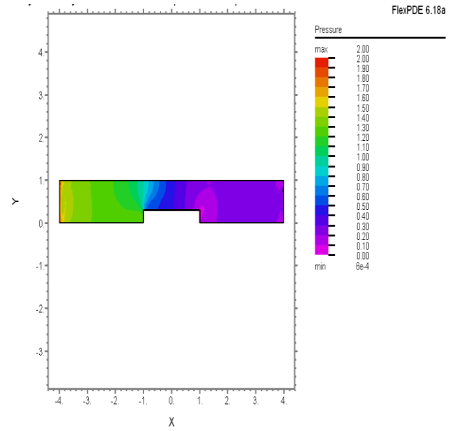
Fig.4: Pressure at h = 0.3
