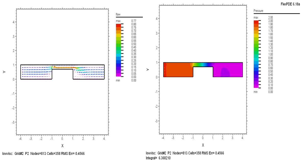
Fig.15:Flow at h = 0.9
