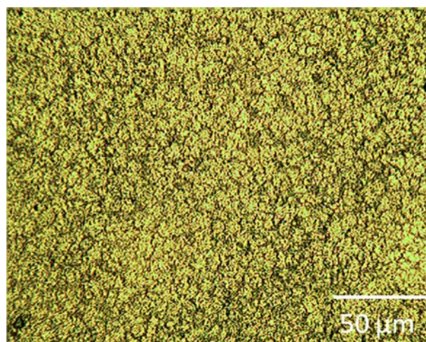
Fig. 6. Optical micrographs showing surface morphology of HVOF sprayed Fe based alloy coating on gray cast-iron.
