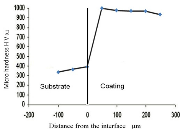
Fig. 7. Micro hardness profile for HVOF sprayed Fe based alloy coating.
