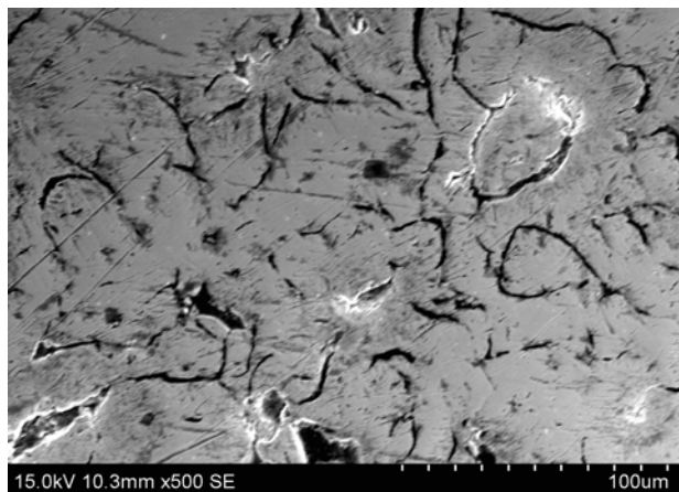
Fig. 1. SEM images of coated Specimen etched with Nital.
