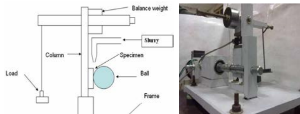
Fig. 2. Schematic diagram of micro abrasion tester.
