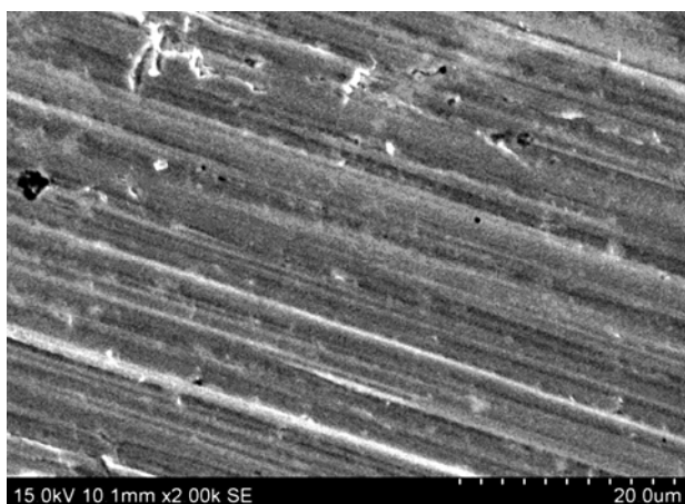
Fig. 10. Wear grooving morphology of coated surface at loading condition.
