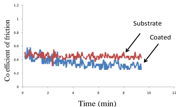
Fig. 11. Online monitoring of coefficient of friction for coating & substrate.
