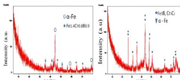
Fig. 8. XRD pattern of FeBCr Powder and FeBCr Coated Surface.
