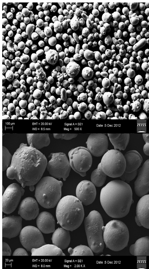
Fig. 3. As-atomized Fe based amorphous powder with particle size between 15-75 \mu\text{m} .
