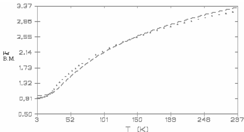
Figure 5. The temperature dependence of the experimental and theoretical values of \mu_{ef} for complex 1 .
