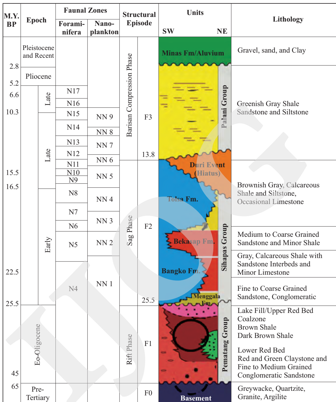
Figure 2. The tectonostratigraphic chart of Central Sumatra Basin (after Heidrick and Aulia, 1993; the Pematang Group is shown in a black circle).
