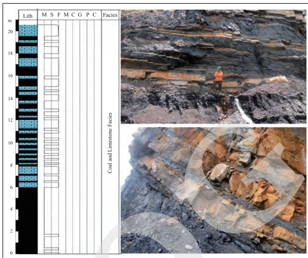
Figure 4. Photograph of interbedded coals and limestones showing the repetition of thickening and coarsening upward cycles; a few limestone wedges out into coal seams.
