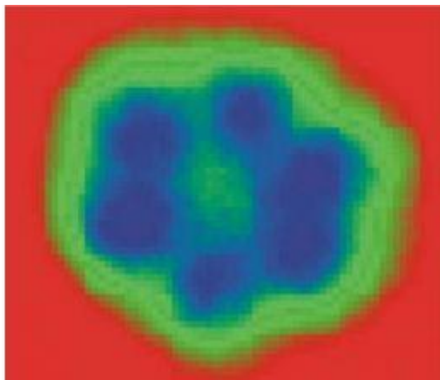
Figure 3. Image of hexamer nanocrystal of ice water (average size \sim 1 nm) by a scanning tunneling microscope after freezing water to 17 K on the hydrophobic metallic plates of Cu and Ag [13].
