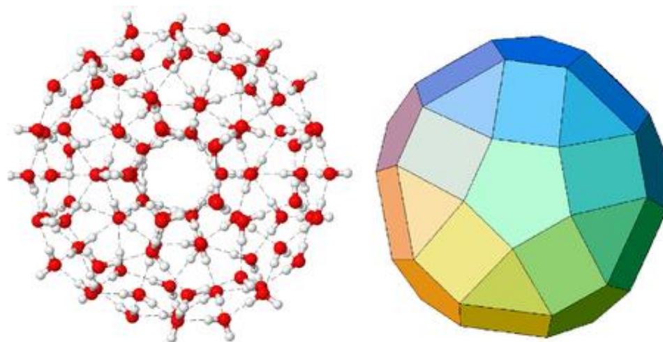
Figure 12. Icosahedron cluster based on 100 H 2 O molecules and the underlying structure according to the M. Chaplin's model
