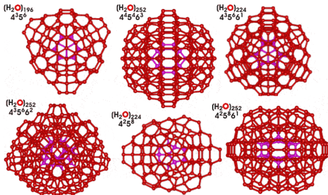
Figure 10. Tetrahedron water clusters (\text{H}_2\text{O})_n with different symmetry ( n = 196, 224, 252 ) [32]
