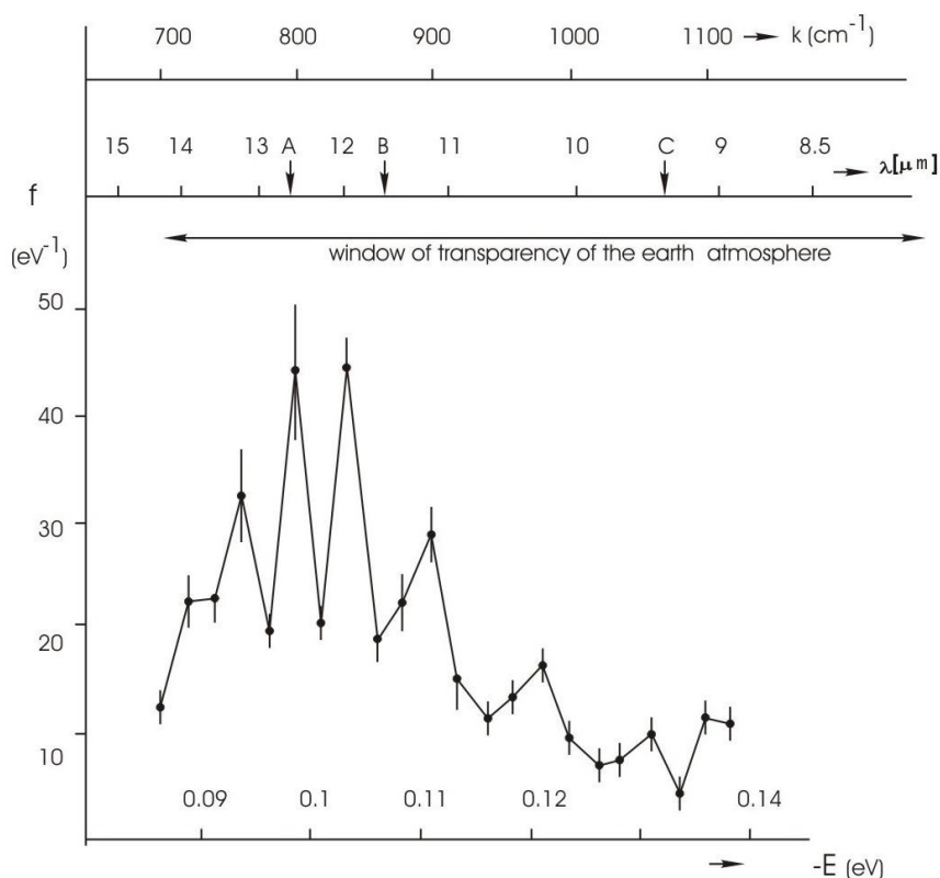
Figure 7. NES-spectrum of deionized water (chemical purity – 99,99 %, pH – 6,5–7,5, total mineralization – 200 mg/l, electric conductivity – 10 \mu\text{S}/\text{cm} ). On the horizontal axis shows the energy of the H...O hydrogen bonds in the associates – E (eV). The vertical axis – energy distribution function – f ( \text{eV}^{-1} ). k – the wave number ( \text{cm}^{-1} ); \lambda – wavelength (mm).
