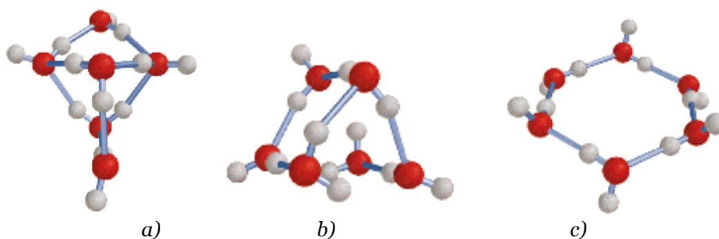
Figure 8. Calculation of small water cluster structures (a–c) with general formula (\text{H}_2\text{O})_n , where n = 6 [29]
