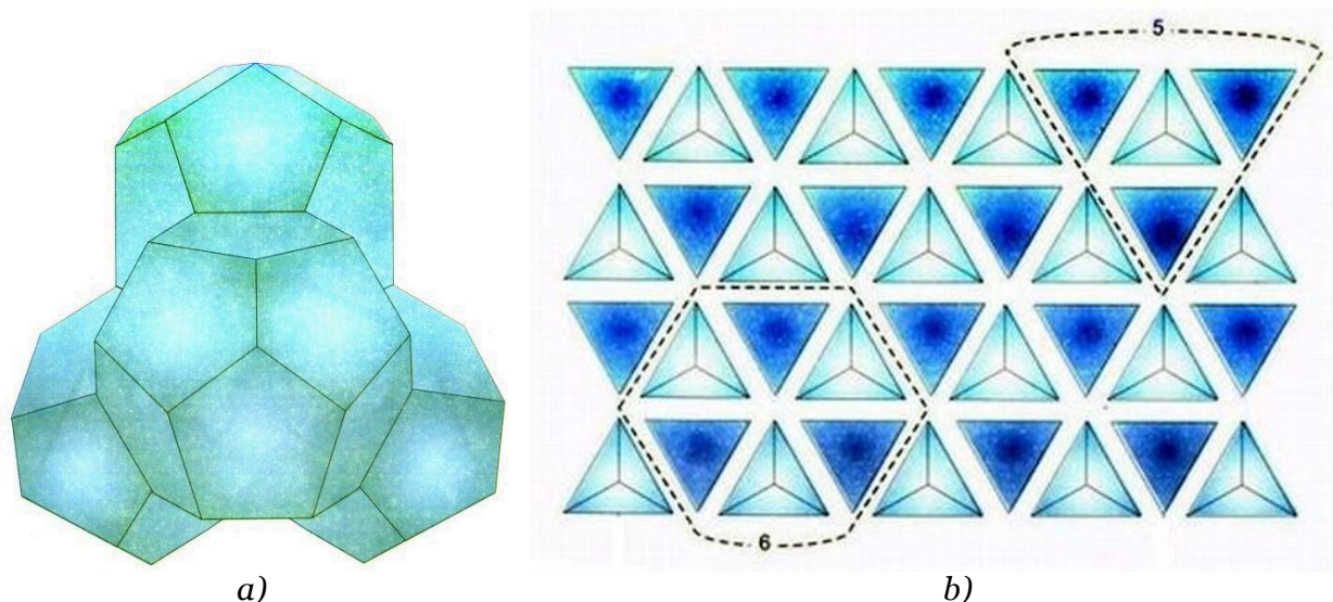
Figure 11. Model of water associate according to the model of S.V. Zenin [33]: a) – associate of 57 H 2 O molecules, tetrahedron of four dodecahedron (“quantum”); b) – bulk packaging of “quanta”
