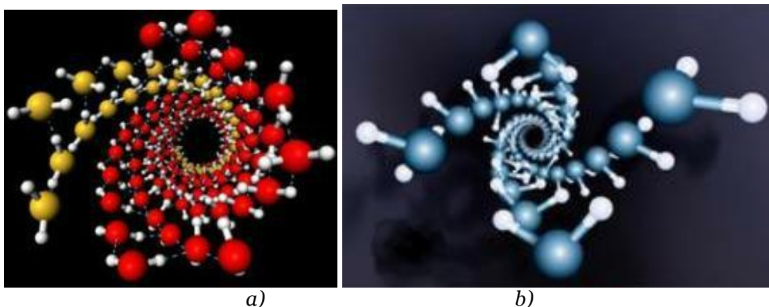
Figure 4. Structures of water crystals in carbon nanotubes according to computer simulations [14] (diameter of nanotubes: 1,35–1,90 nm; pressure: 10–40000 atm; temperature: -23 °C): a) – a general view of the crystal structure of water in nanotubes, b) – the inner wall of the structure of water
