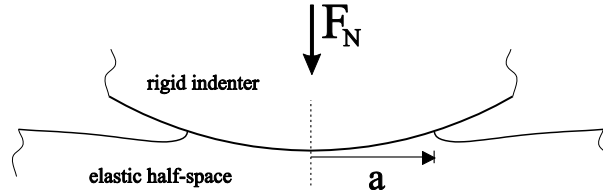
Fig. 1 Qualitative presentation of an adhesive contact between a rigid, curved body and an elastic half-space
