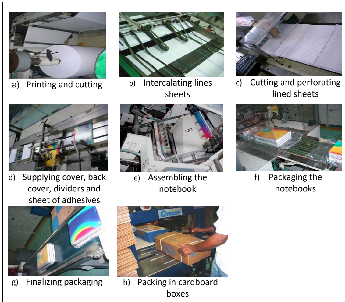
Figure 3: Script for manufacturing university notebooks Source: Tilibra (2007)
