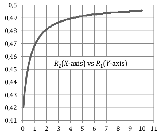
Fig. 8. Relationship between R_2 and R_1 for single moving load.
