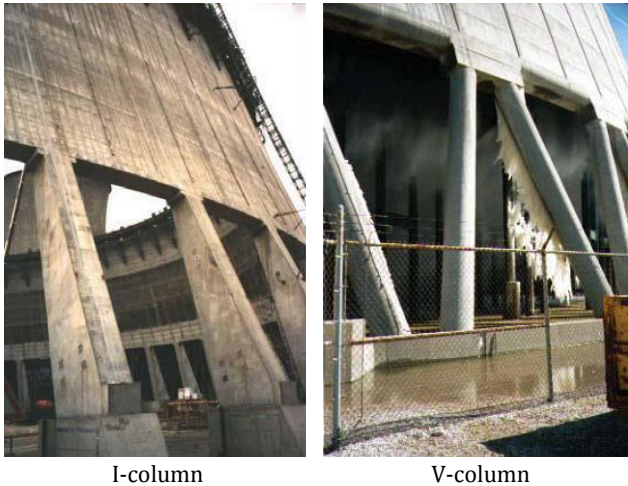
Fig. 1. Cooling tower column systems.
