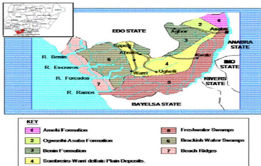
Fig. 1: Aerial distribution of Quaternary- Holocene deposits and the Benin Formation in part of the western Niger Delta. The map of Nigeria is shown as an inset. (Modified from Akpoborie et al., 2011).
