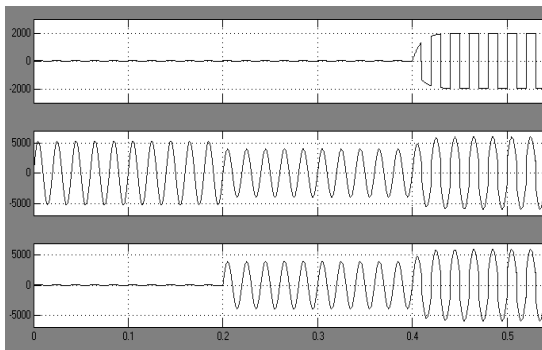
Fig.5 Voltage across external, LOAD-1 &LOAD-2 waveforms
