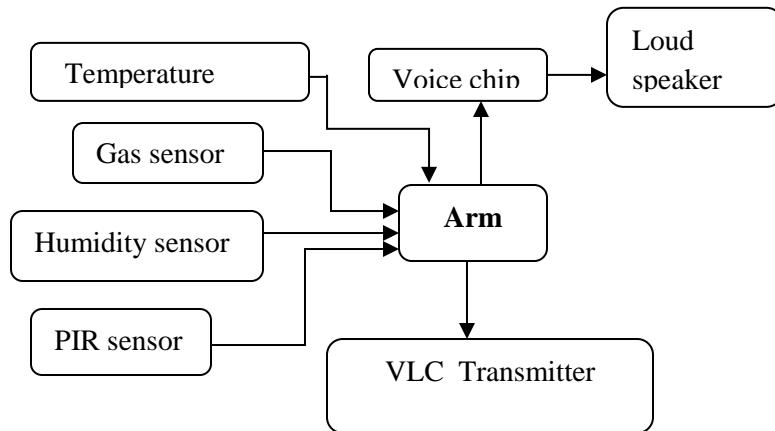
Fig 7.1.1.1 Proposed Block Diagram for Mine Section
