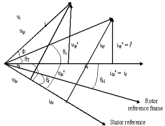
Phasor diagram of vector controller
