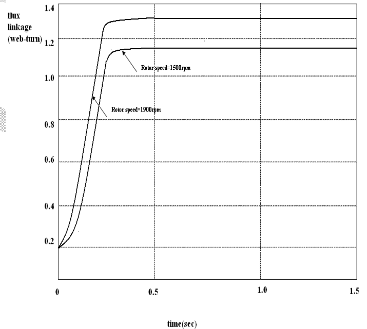
Flux linkage at different rotor speeds of the induction generator
