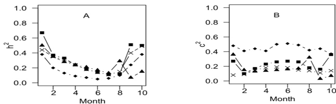
Figure 2. Estimates of heritability ( h^2 , A ) and proportion of phenotypic variance due to the permanent environment ( c^2 , B ) for milk yield LEG3,5_4 (♦), fat yield LEG3,4_4 (■), protein yield LEG3,4_4 (▲), and mozzarella production LEG3,4_4 (x).
