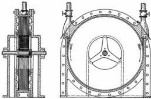
Fig 1. Telsa Turbine
