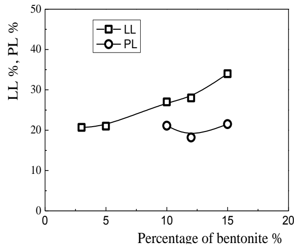
Fig 2. Relationship between Atterberg limits and bentonite content.
