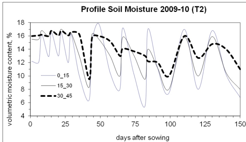
Fig. 2(b). Profile soil moisture content for T 2 (40% MAD) during 2009-10.
