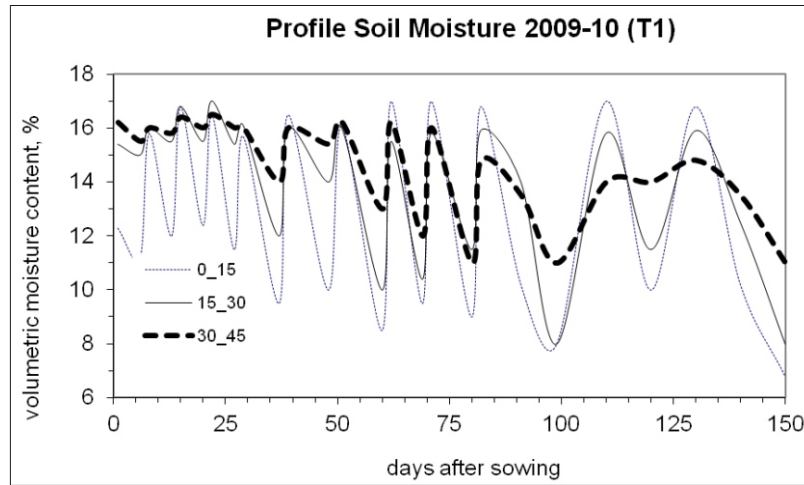
Fig. 1(b). Profile soil moisture content for T 1 (20% MAD) during 2009-10.
