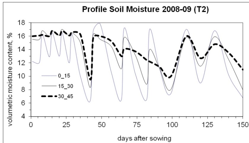
Fig. 2(a). Profile soil moisture content for T 2 (40% MAD) during 2008-09.
