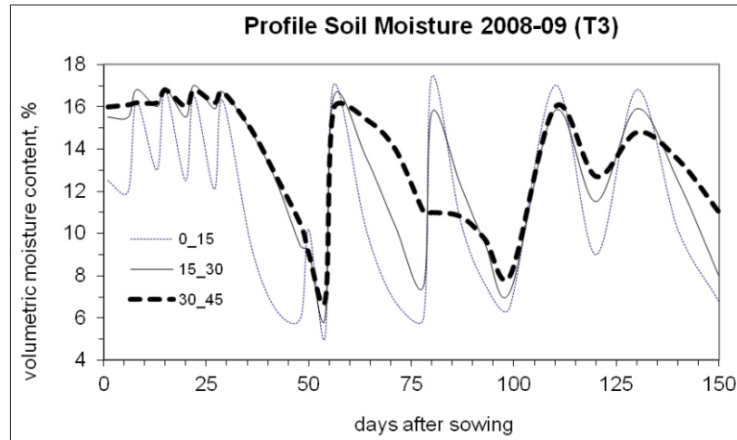
Fig. 3(a). Profile soil moisture content for T_3 (60% MAD) during 2008-09.
