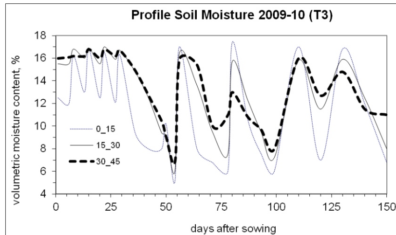
Fig. 3(a). Profile soil moisture content for T_3 (60% MAD) during 2009-10.
