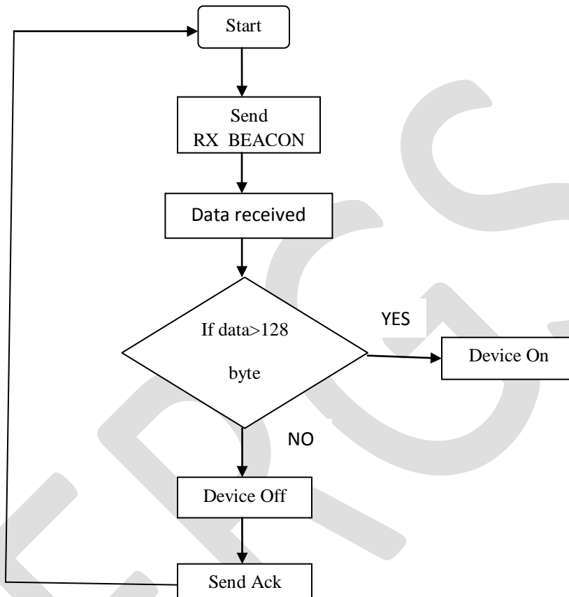
Fig.3. Receiver Flow Diagram
