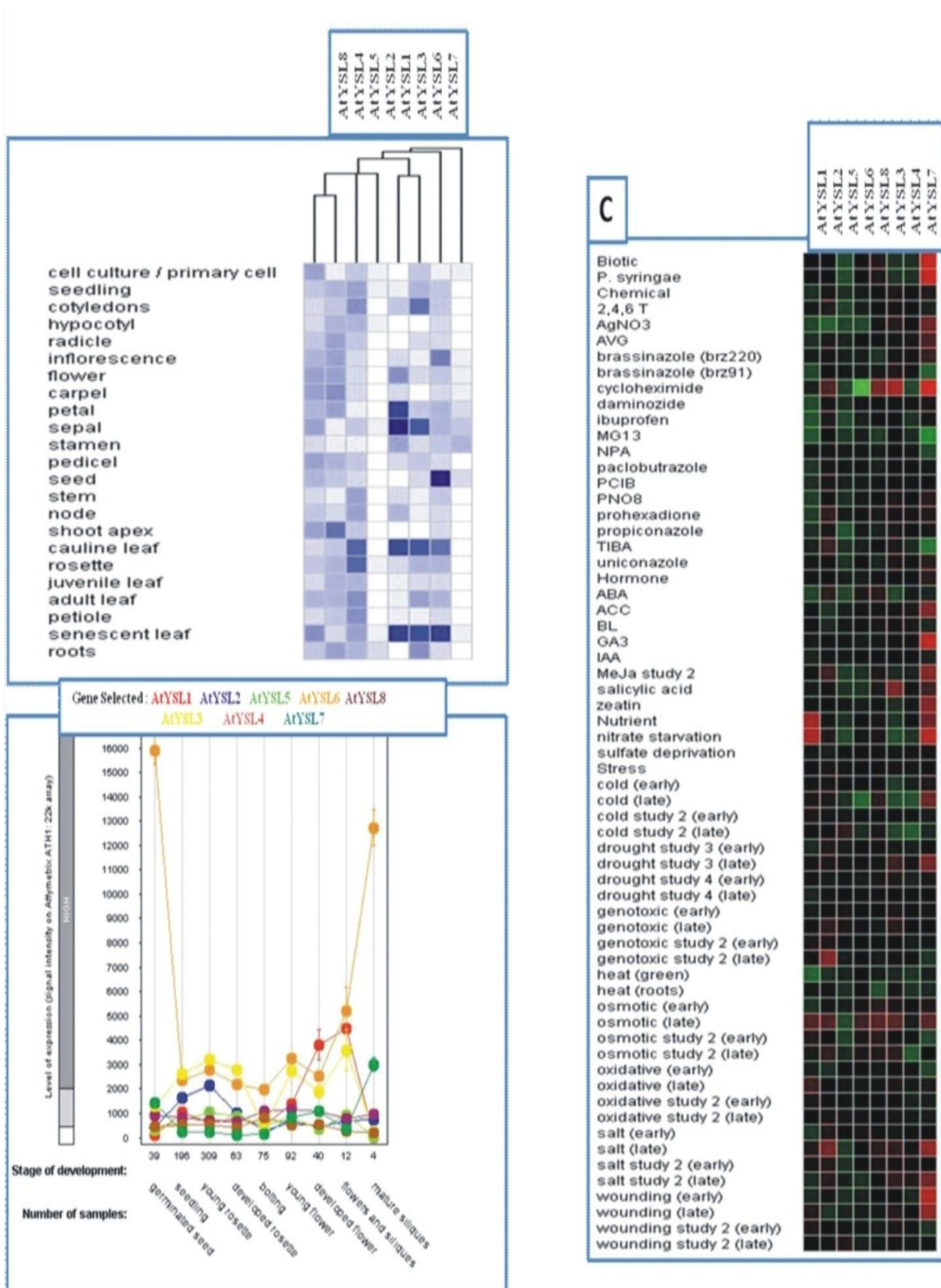
Fig. 9- Digital expression pattern analysis of YSL genes in Arabidopsis . Based on public microarray data, digital expression pattern was performed by Genevestigator. Arabidopsis YSL family genes expression patterns at different development stages, in anatomical tissues and under different stimulus are shown. Hierarchical clustering was played in data analysis as shown in figure A, B and C.
