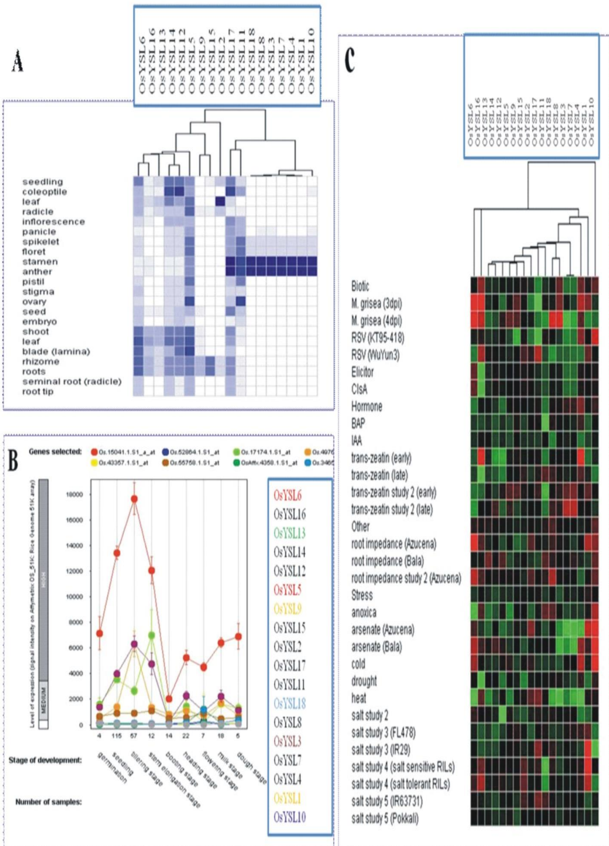
Fig. 8- Digital expression pattern analysis of YSL genes in Rice. Based on public microarray data, digital expression pattern was performed by Genevestigator. Rice YSL family genes expression patterns at different development stages, in anatomical tissues and under different stimulus are shown. Hierarchical clustering was played in data analysis as shown in figure A, B and C.
