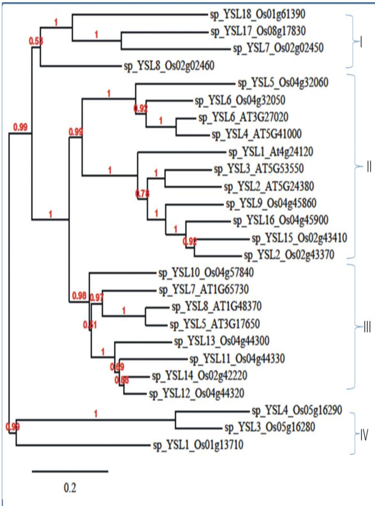
Fig. 1- Combined phylogenetic relationship between OsYSL and AtYSL proteins. Bootstrap values from 1000 replicate are indicated at each node. Scale bar represents 0.2 amino acid substitution per site. The protein on the tree can be divided into four distinct subfamilies (I-IV).
