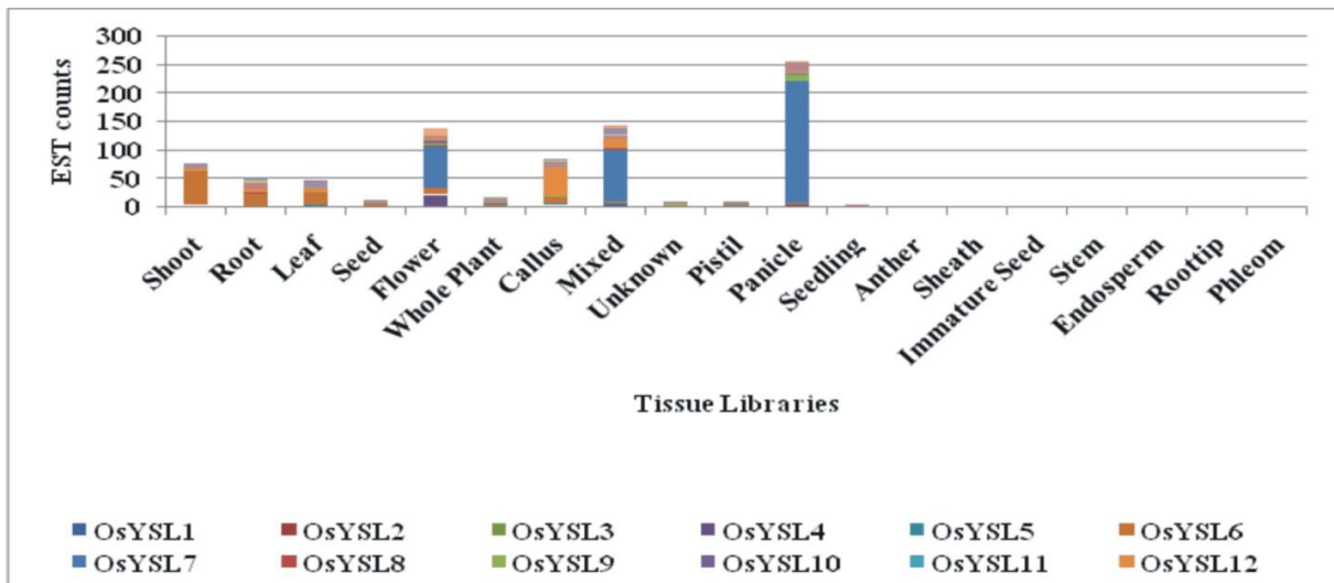
Fig. 5- EST count distribution in different tissue libraries concerned with different YSL genes in rice.
