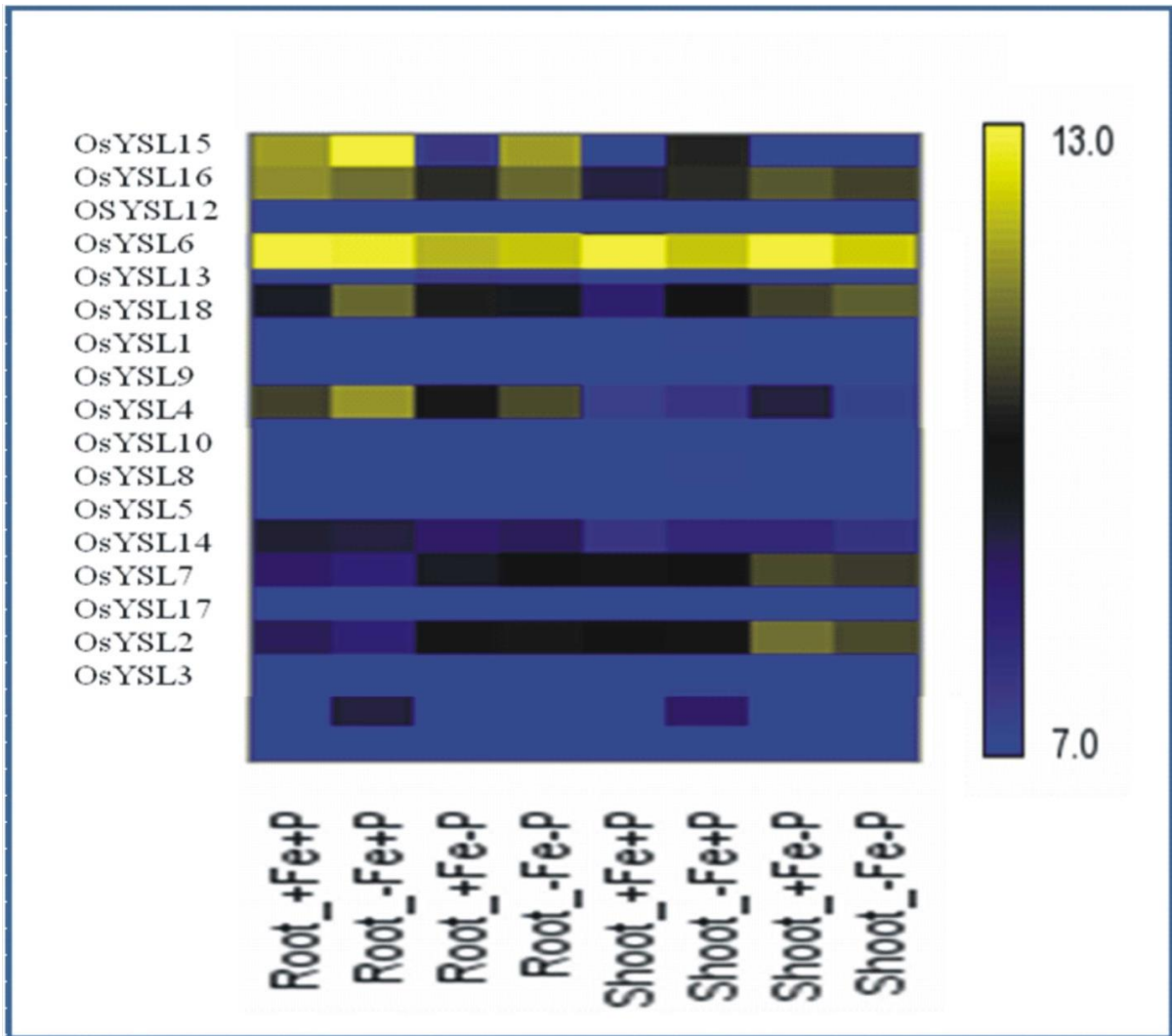
Fig.10- Expression of OsYSL genes under the iron and phosphorous interaction in root and shoot tissues.
