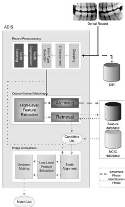
Fig.1- ADIS Block Diagram.
