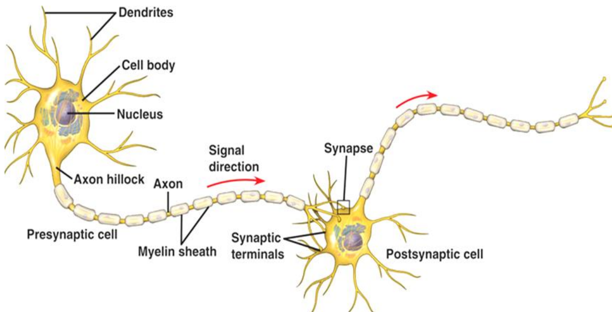
Figure 1. Neuron structure.
