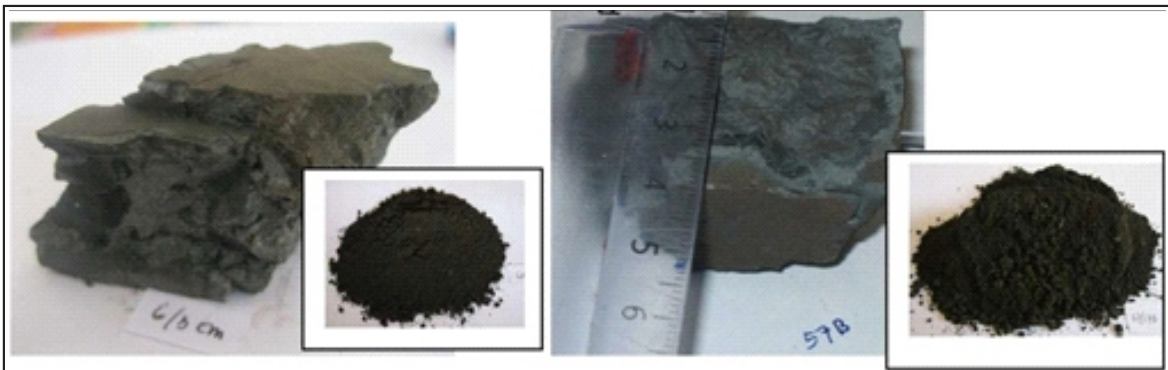
Figure 7. Photograph of Manganese layer handspecimen with physical properties: blackish grey, weak, less massive, lighter than Mn ore in Figure 6d (pyrolusite), brownish black-pale reddish brown powder colour. Based on those characteristics, it may meet with the characteristics of groutite.
