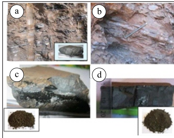
Figure 6. Photograph of (a) and (b). Outcrops of interbedded manganese layers and claystone/siltstone. (c) and (d). Hand-specimen of manganese layers identified as pyrolusite.
