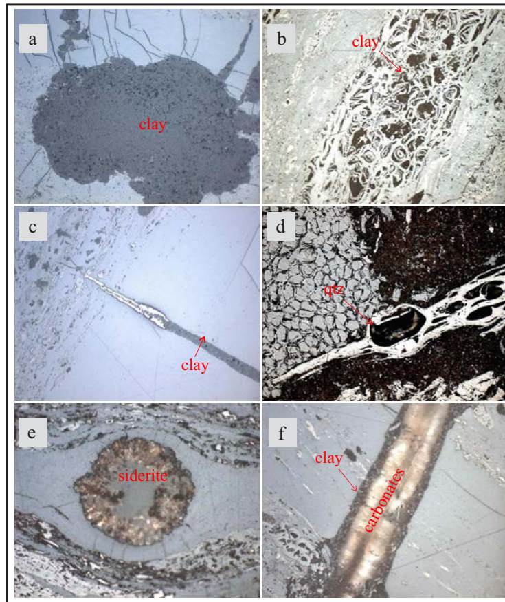
Figure 5. Photomicrographs showing mineral matter occurrences in the South Walker Creek coals (reflected light, oil immersion); a: Massive bodies of clay minerals in telocollinite, 20x, 11852-7; b: Clay minerals infilling cell lumens in fusinite, 20x, 11424-13; c: Clay minerals in cleat infillings of vitrinite macerals, 20x, 11852-2; d: Fine rounded crystal of quartz (qtz) in a cell lumen infilling of fusinite, 20x, 11424-27; e: Siderite nodule in a vitrinite band, 50x, 11424-22; f: Carbonate minerals in association with clay in cleats, 20x, 11852-10.
