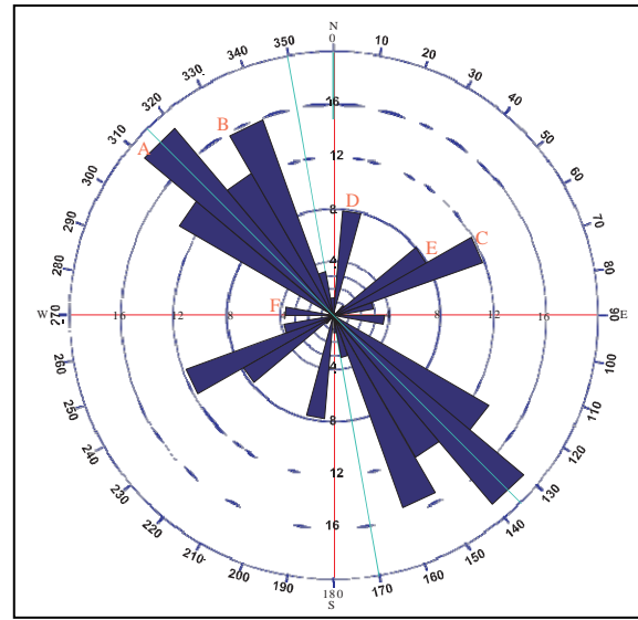
Figure 13. A rose diagram as the measurement result of length version azimuth of fault lineament showing an active fault zonation in Mahawu, ranging between N 120° E - N 160° E and N 300° E - N 340° E.
