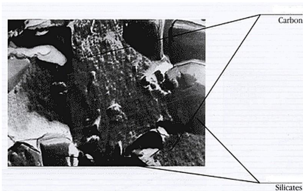
Figure 2. Structure of schungite rock obtained by TEM method. Scanning area 100 \times 100 nm, resolution 0,5 nm, magnification 300000 times. The arrows show the silicate framework of fine dispersed quartz with the size 1–10 \mu\text{m} , and uniformly distributed carbon
