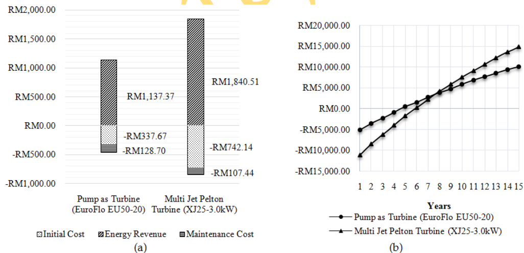
Figure 2: (a) Annual life cycle cost for PAT and Multi Jet Pelton (b) Cash Flow for PAT and Multi Jet Pelton
