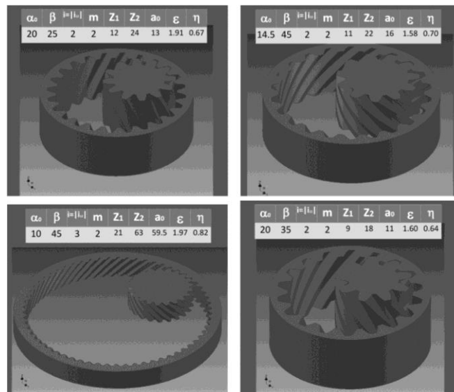
Fig. 9 Validated examples of internal gearing
