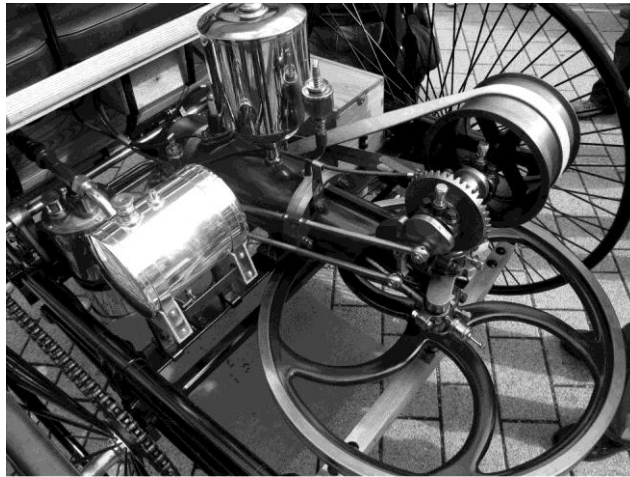
Fig. 4 The Benz patent
