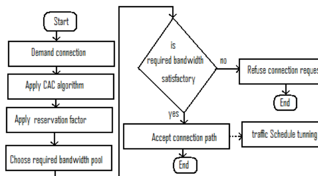
Figure 1: The Flow Chart for Request Connection
