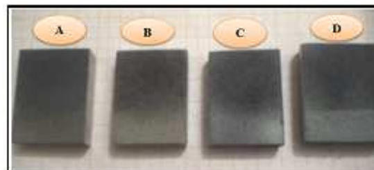
Figure 10: Photograph of Specimens after Erosion Wear Test A: AZ, 80mm, 30° B: AZ, 50mm, 90° C: AT, 50mm, 30° D: AT 80 mm, 90°
