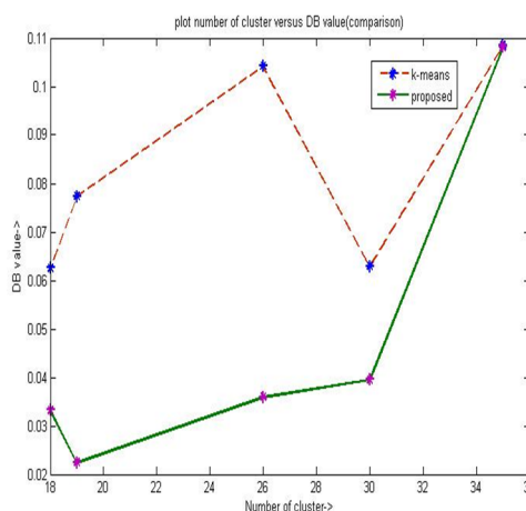
Fig. 11- DB-index comparison for ANCR
