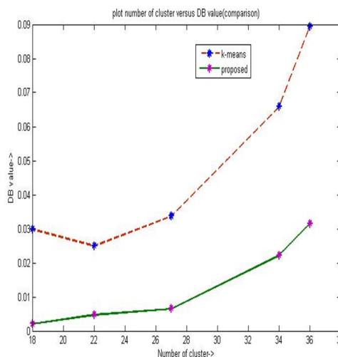
Fig. 9- DB-index comparison for GSE16415
