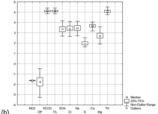
Fig. 5-Box Plots for Ln-Transformed Variables (Rosetta & Damietta Branches during August)
