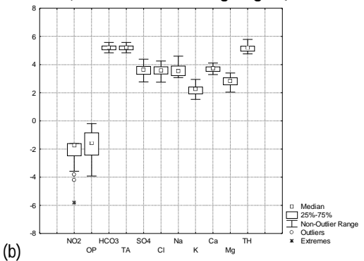
Fig. 4-Box Plots for Ln-Transformed Variables (Rosetta & Damietta Branches during February)
