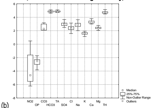
Figure 3: Box Plots for Ln-Transformed Variables (Main Nile Sites during August)
