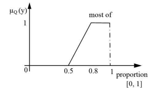
Figure 3: Linguistic relative quantifier most of . (Zapletal et al., 2023)
