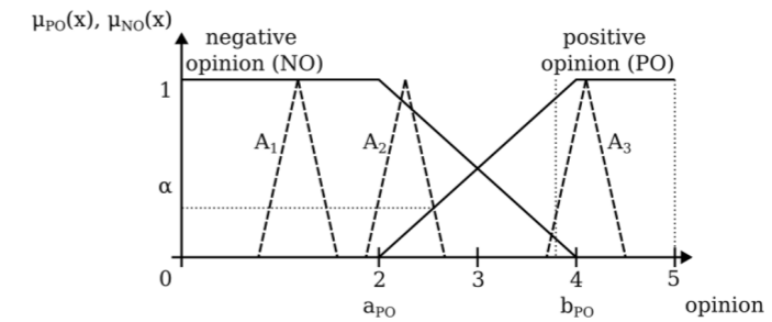
Figure 2: Definition of positive and negative opinion and example of a possibility measure for three fuzzy numbers: \text{Pos}(A_1, PO) = 0 , \text{Pos}(A_2, PO) = \alpha , \text{Pos}(A_3, PO) = 1 .
