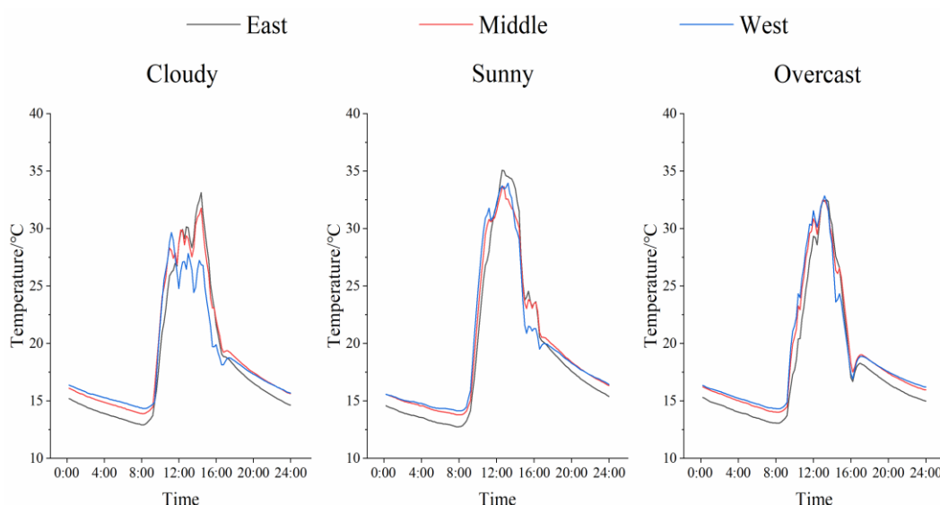
Fig. 3 - Graph of daily variation of temperature in the solar greenhouse
