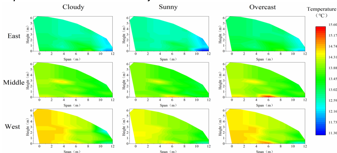
Fig. 4 - Cross-sectional temperature distribution of the solarium during extreme low temperatures
