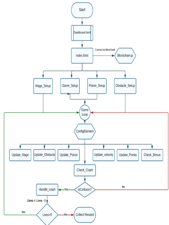
Figure A.2.1.Back End Implementation
