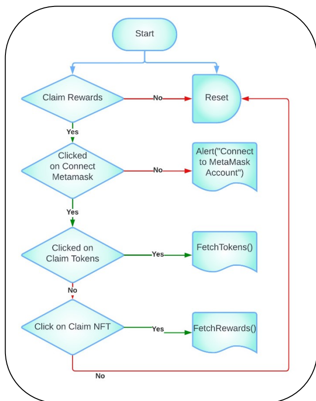
Figure A.3.1. Blockchain Reward Collection Algorithm flowchart
