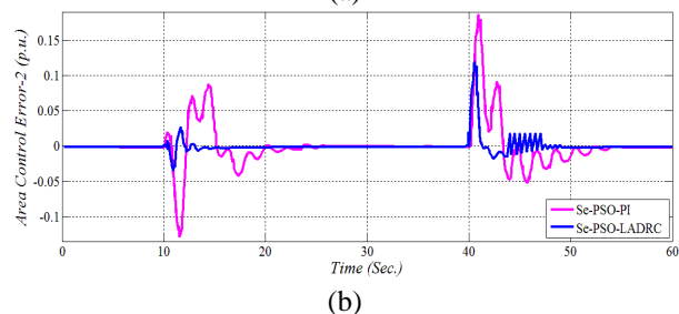
Figure. 7 Area-2 under pumping mode: (a) Frequency deviation response and (b) ACE response
