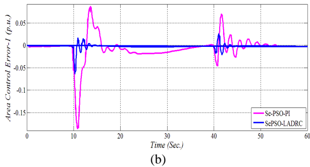
Figure. 6 Area-1 under pumping mode: (a) Frequency deviation response and (b) ACE response
